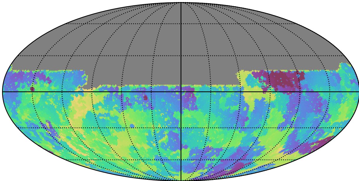
too_100_1v3.4_10yrs All sky u band: Min skyBrightness
