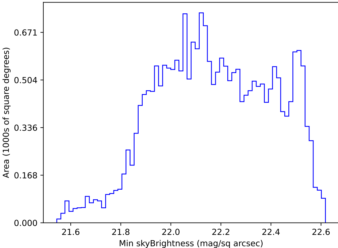
too_100_1v3.4_10yrs All sky u band: Min skyBrightness
