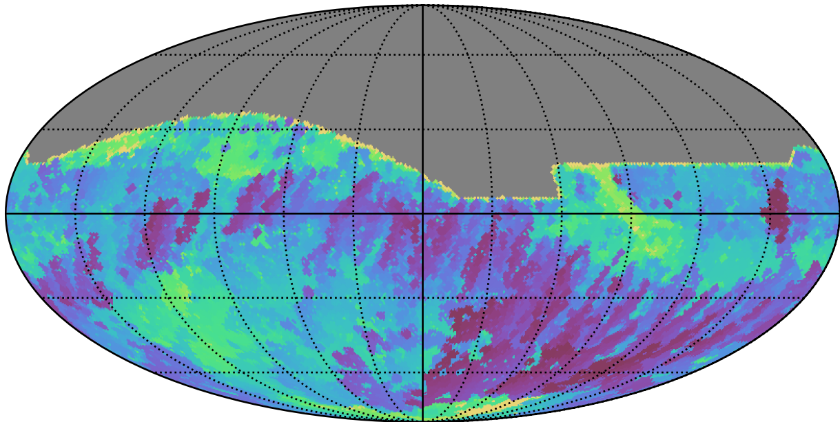
too_100_1v3.4_10yrs All sky r band: Min skyBrightness
