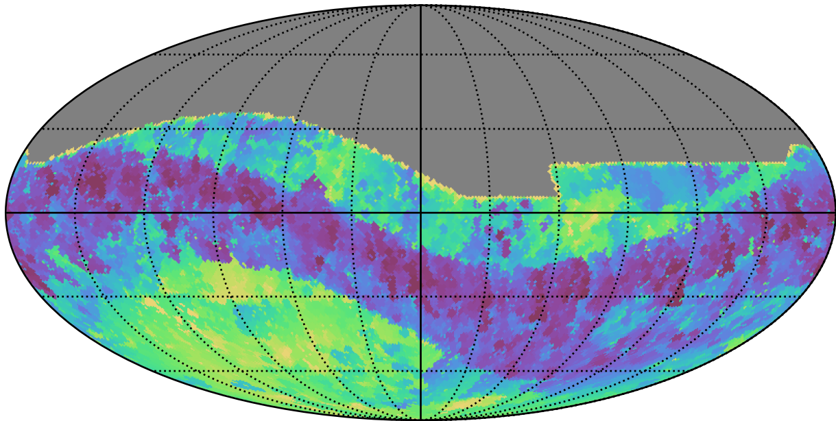
too_100_1v3.4_10yrs All sky i band: Min skyBrightness
