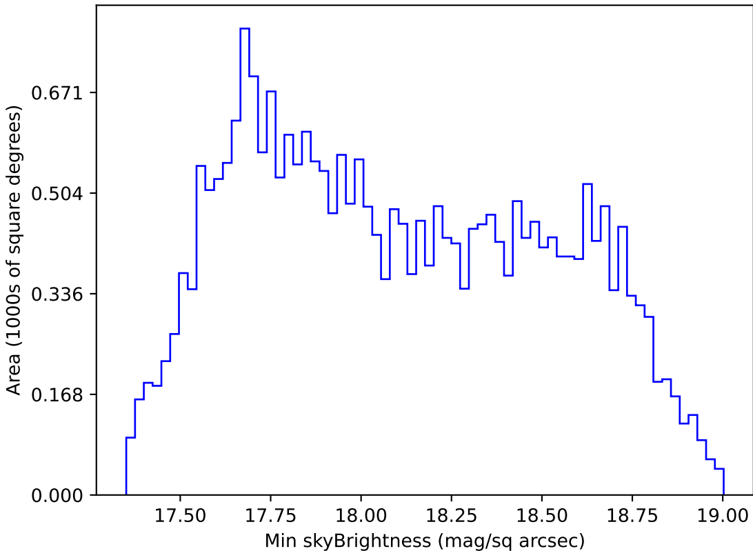
too_100_1v3.4_10yrs All sky i band: Min skyBrightness
