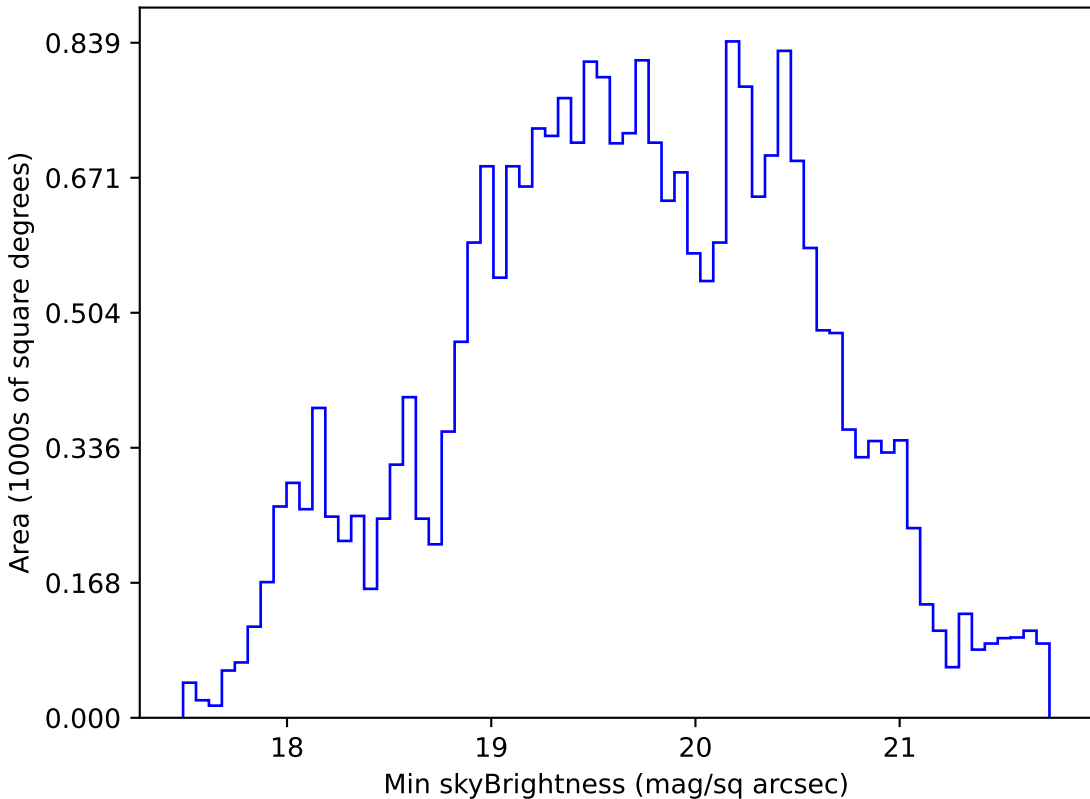
too_100_1v3.4_10yrs All sky g band: Min skyBrightness
