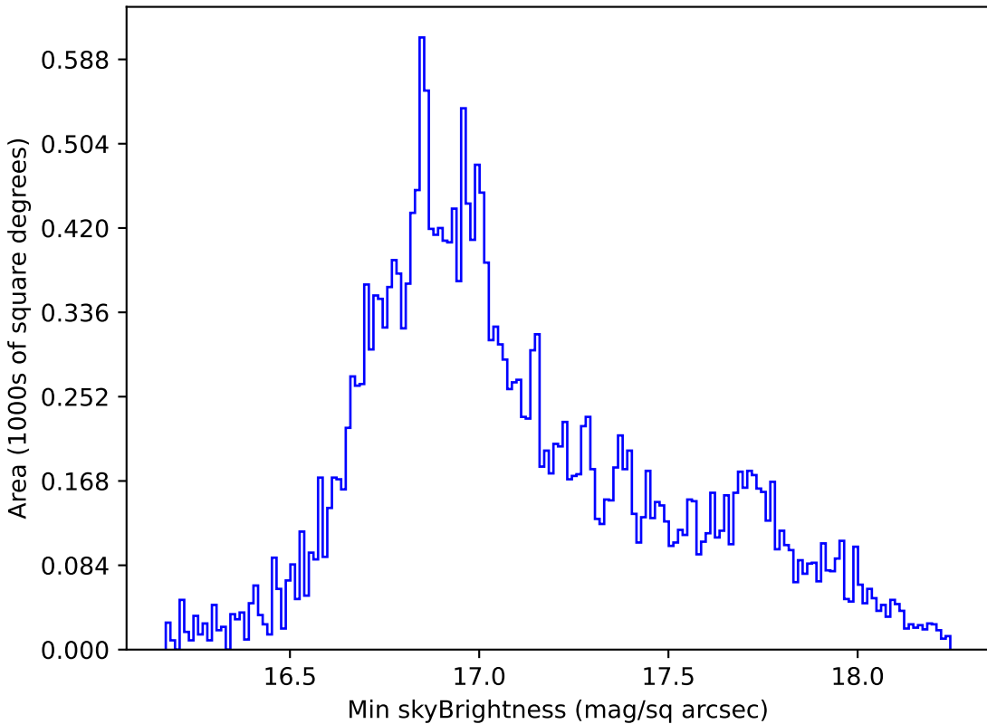
too_100_1v3.4_10yrs All sky all bands: Min skyBrightness
