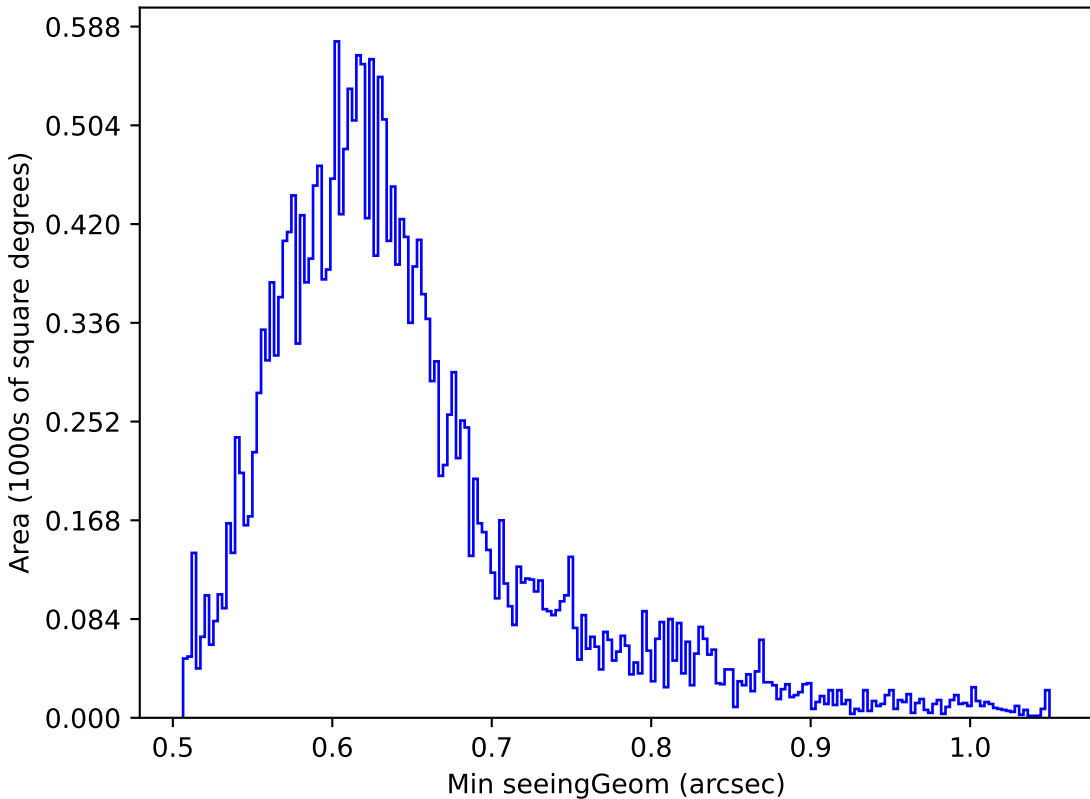
too_100_1v3.4_10yrs Yr 1 z band: Min seeingGeom
