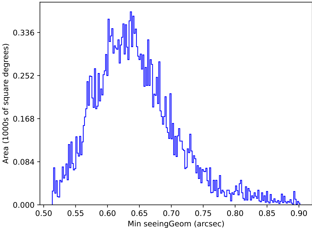
too_100_1v3.4_10yrs Yr 1 y band: Min seeingGeom
