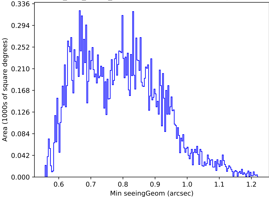
too_100_1v3.4_10yrs Yr 1 u band: Min seeingGeom
