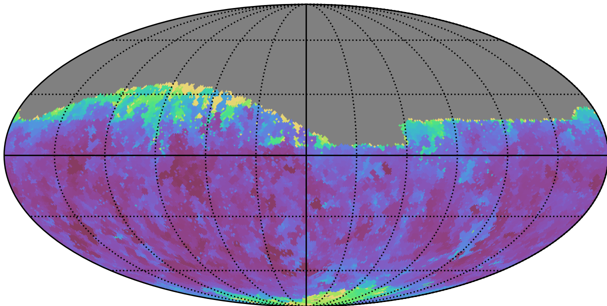
too_100_1v3.4_10yrs Yr 1 r band: Min seeingGeom
