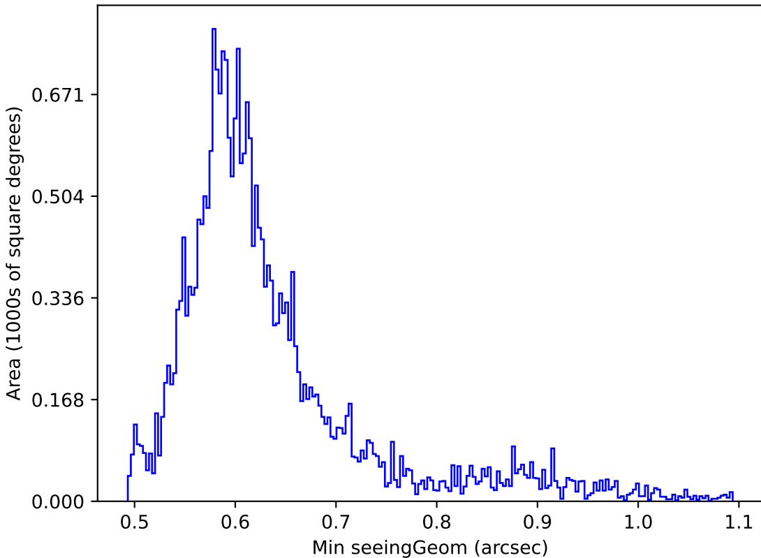
too_100_1v3.4_10yrs Yr 1 i band: Min seeingGeom
