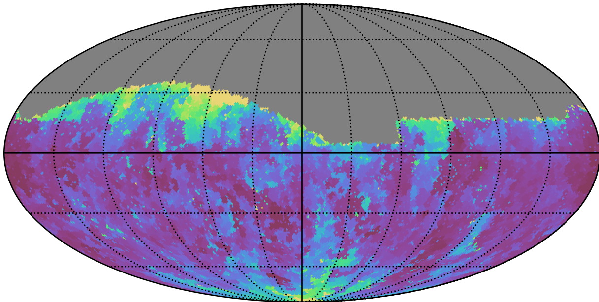
too_100_1v3.4_10yrs Yr 1 g band: Min seeingGeom
