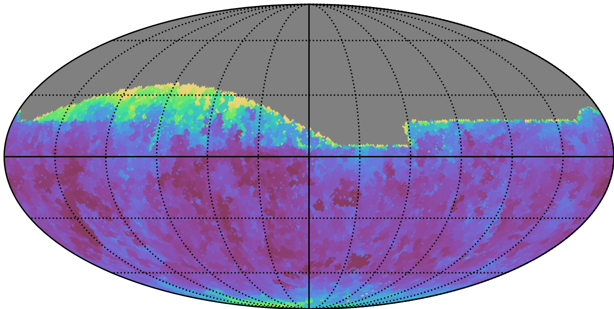
too_100_1v3.4_10yrs Yr 1 all bands: Min seeingGeom
