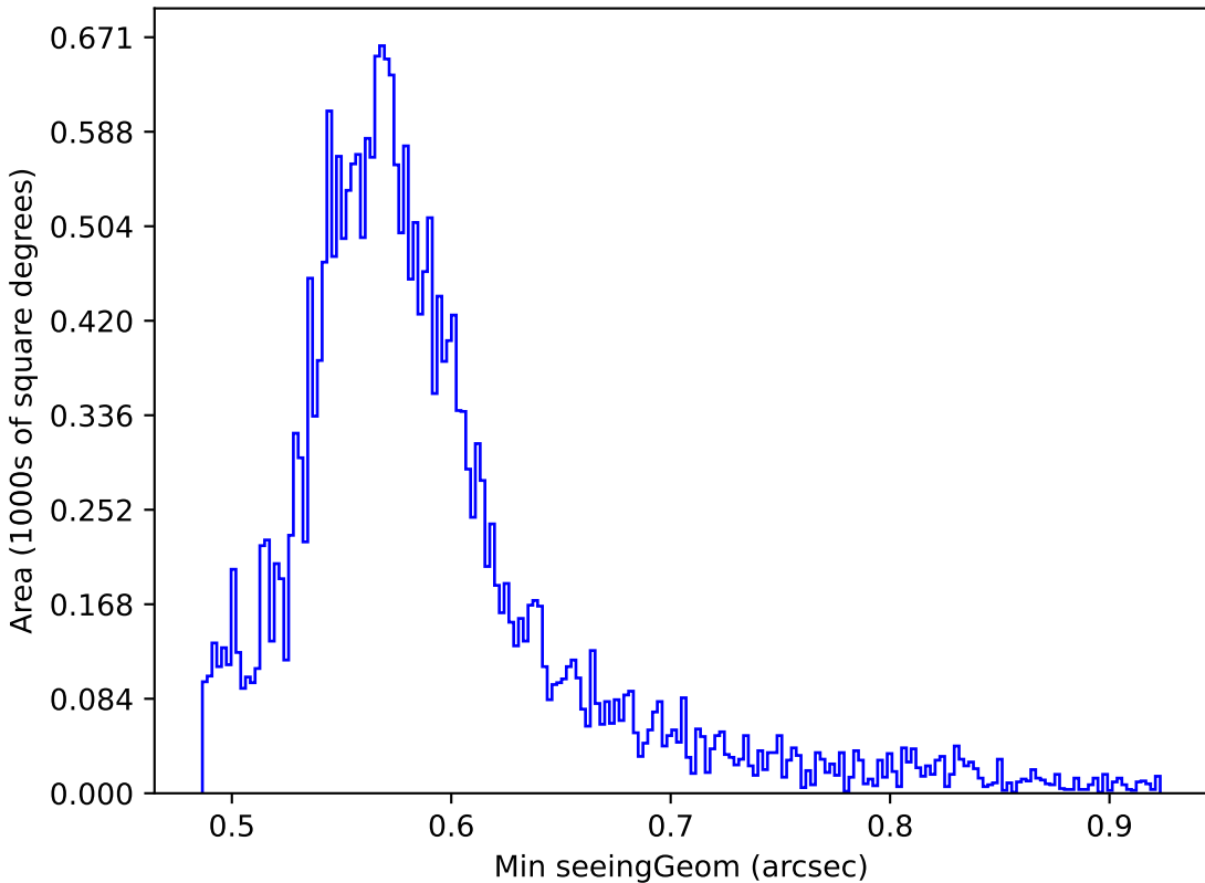
too_100_1v3.4_10yrs Yr 1 all bands: Min seeingGeom
