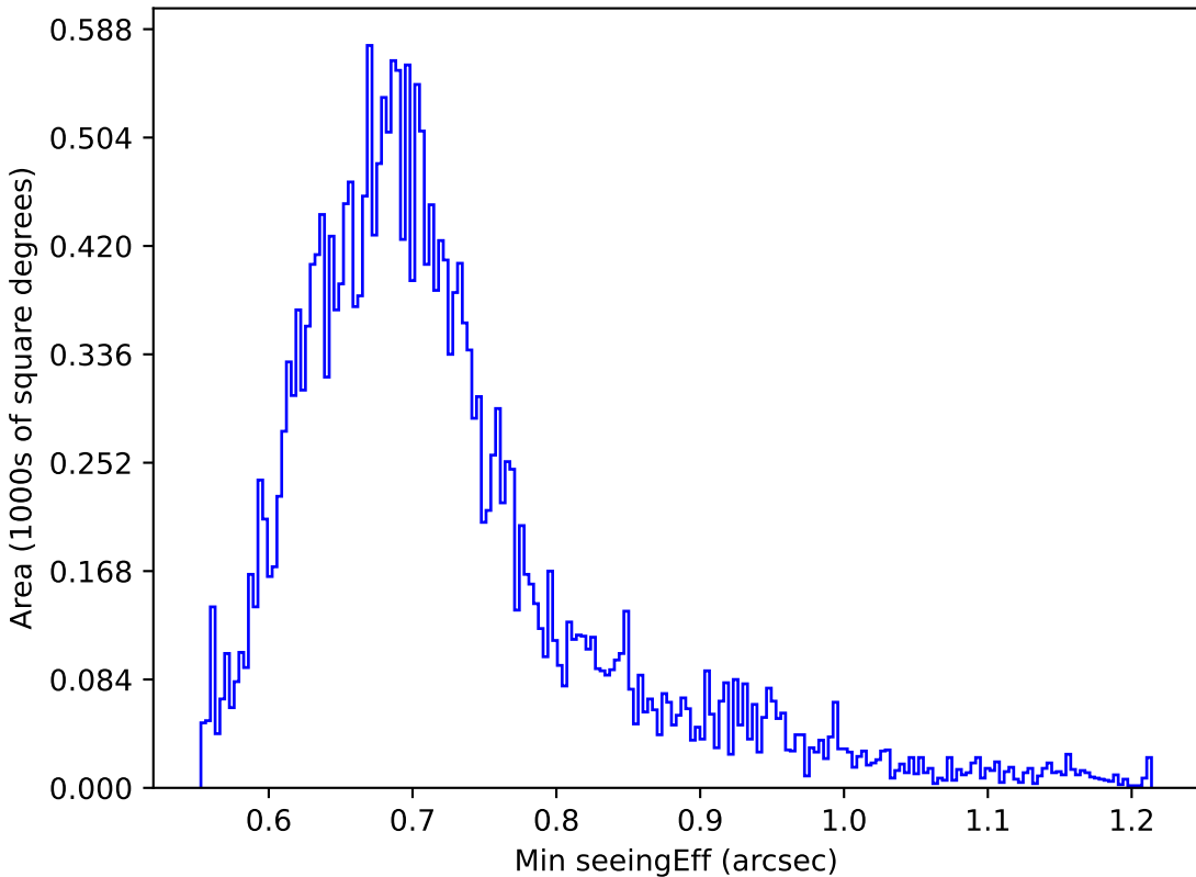
too_100_1v3.4_10yrs Yr 1 z band: Min seeingEff
