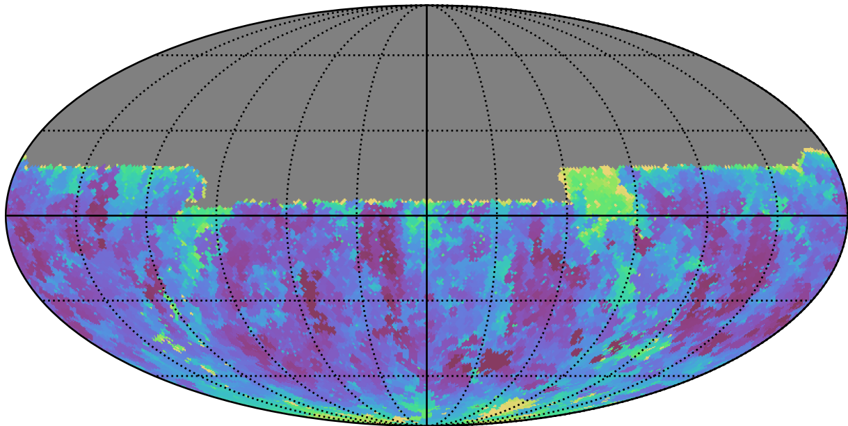
too_100_1v3.4_10yrs Yr 1 y band: Min seeingEff
