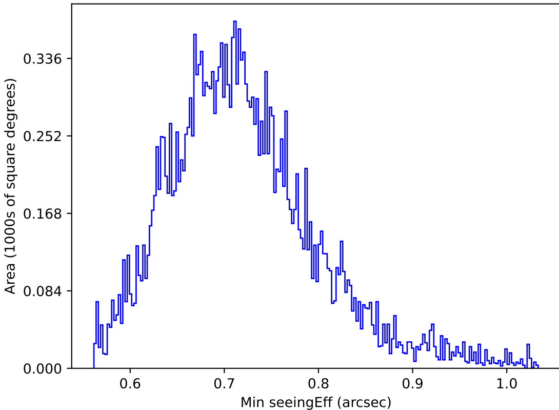
too_100_1v3.4_10yrs Yr 1 y band: Min seeingEff
