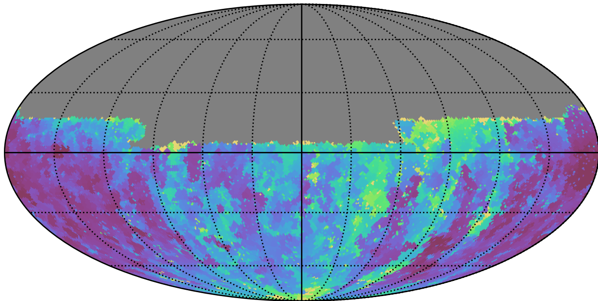
too_100_1v3.4_10yrs Yr 1 u band: Min seeingEff
