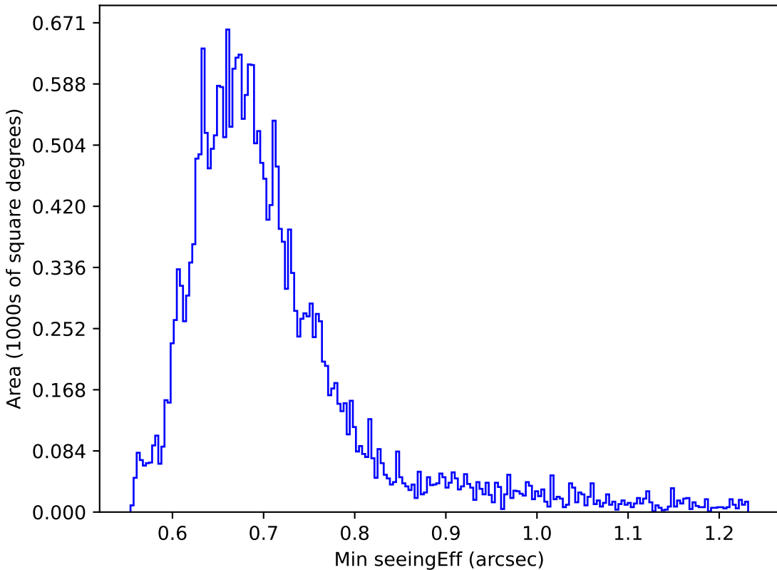
too_100_1v3.4_10yrs Yr 1 r band: Min seeingEff
