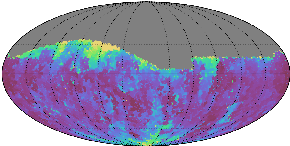
too_100_1v3.4_10yrs Yr 1 g band: Min seeingEff
