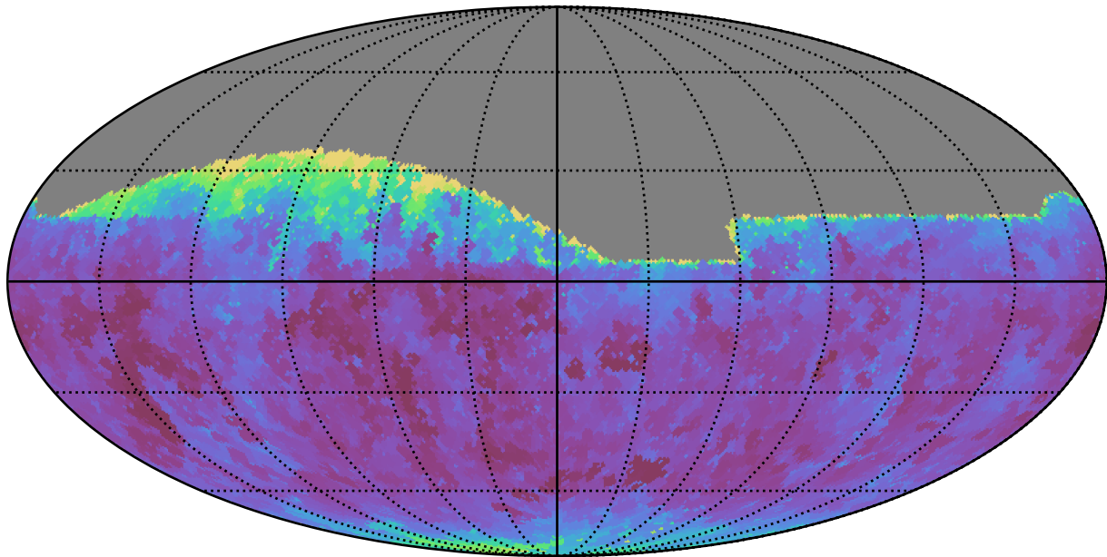
too_100_1v3.4_10yrs Yr 1 all bands: Min seeingEff
