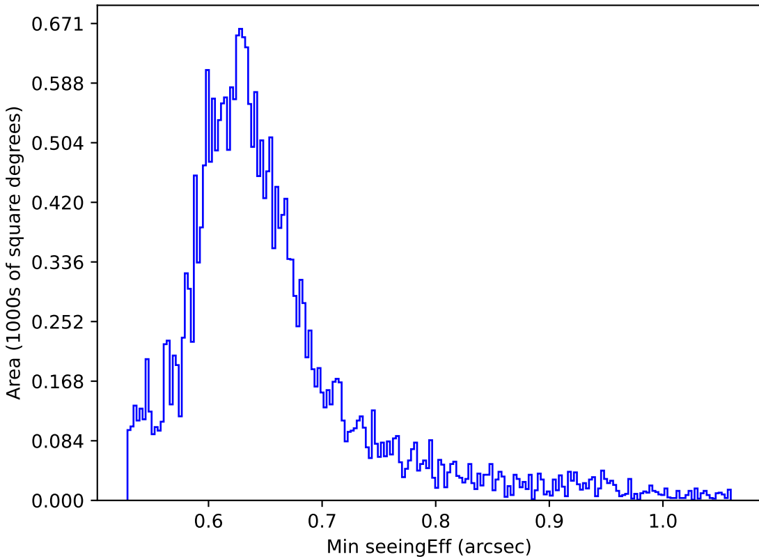
too_100_1v3.4_10yrs Yr 1 all bands: Min seeingEff
