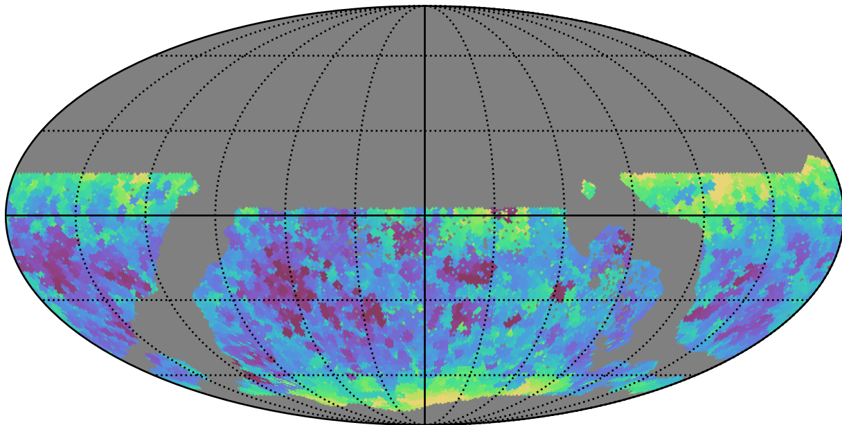
too_100_1v3.4_10yrs WFD z band: Min seeingEff
