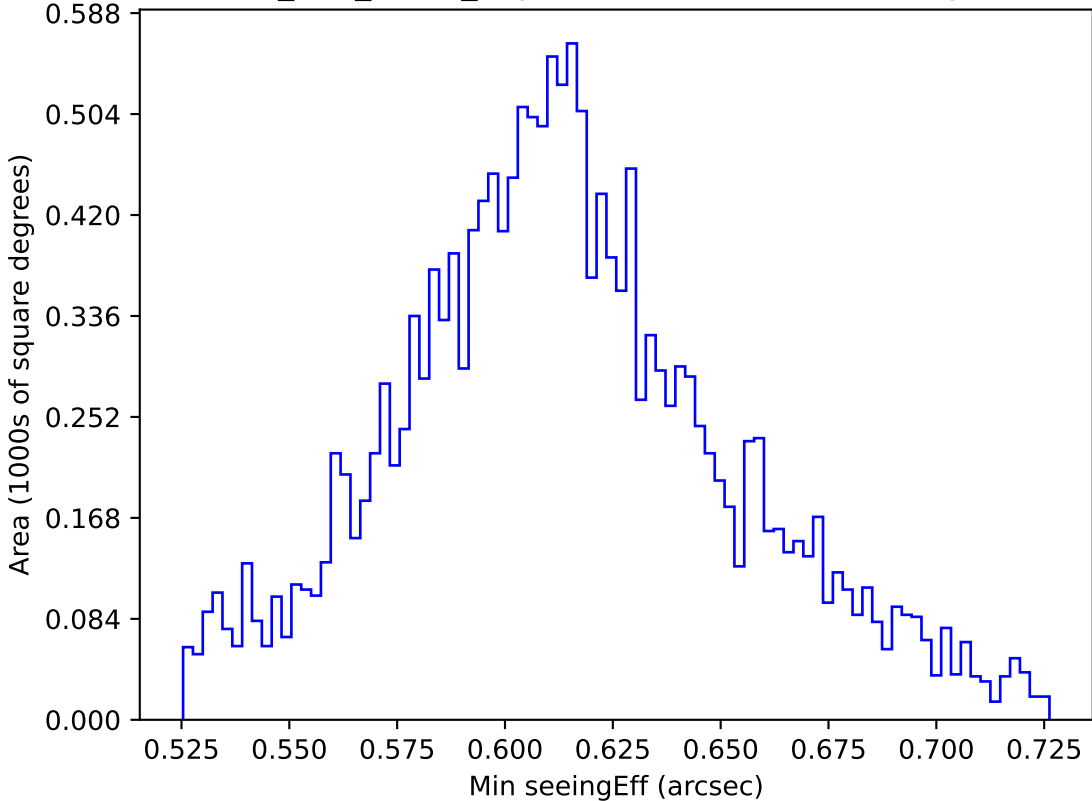
too_100_1v3.4_10yrs WFD z band: Min seeingEff
