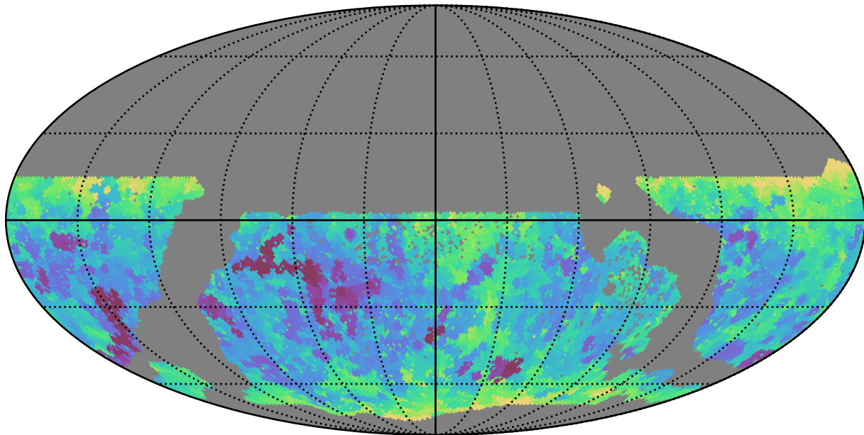
too_100_1v3.4_10yrs WFD y band: Min seeingEff
