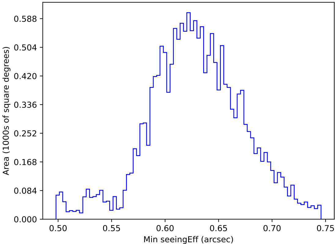
too_100_1v3.4_10yrs WFD y band: Min seeingEff
