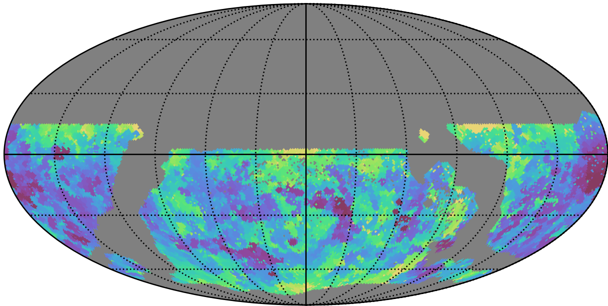
too_100_1v3.4_10yrs WFD u band: Min seeingEff
