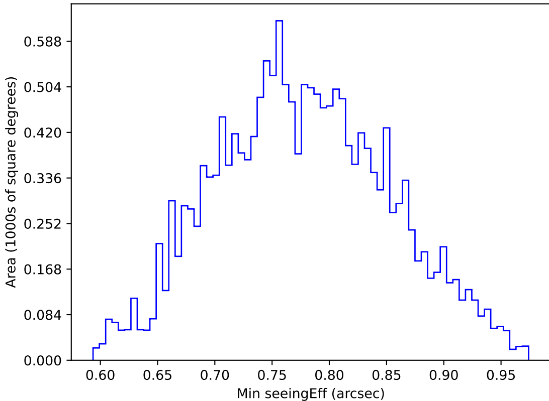
too_100_1v3.4_10yrs WFD u band: Min seeingEff
