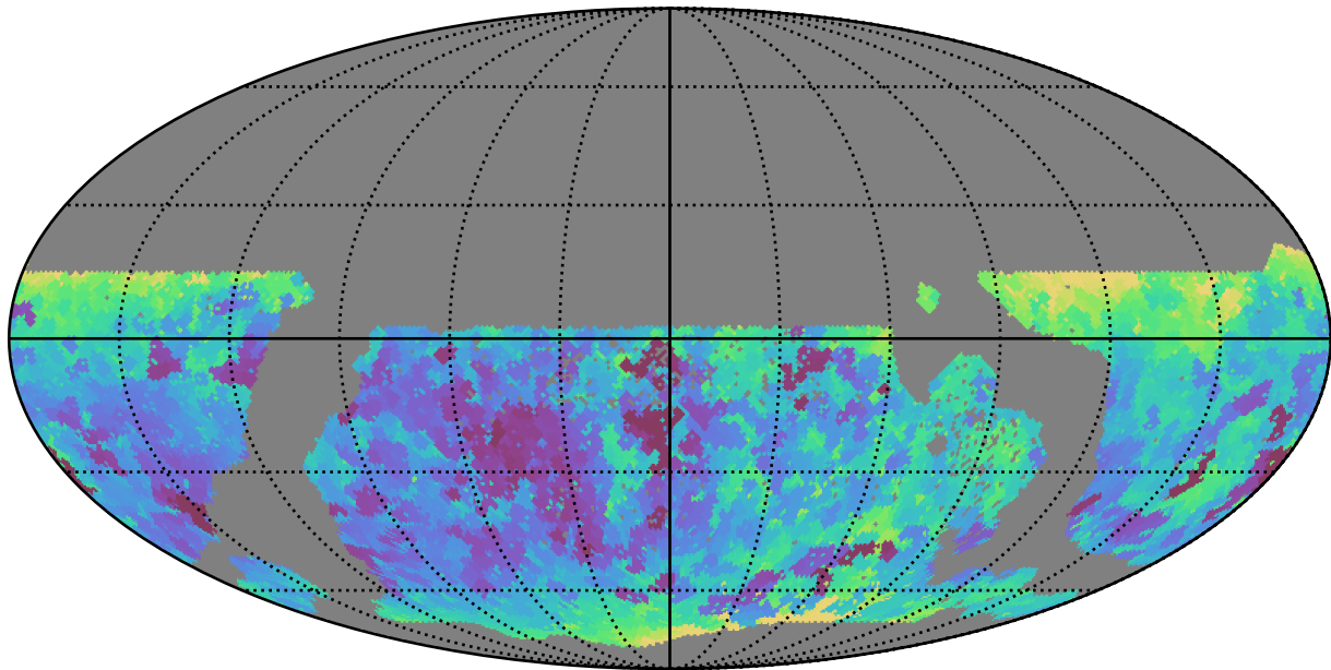
too_100_1v3.4_10yrs WFD r band: Min seeingEff
