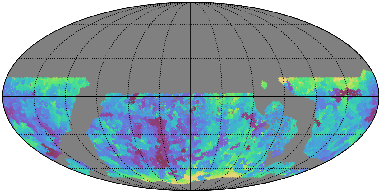
too_100_1v3.4_10yrs WFD g band: Min seeingEff
