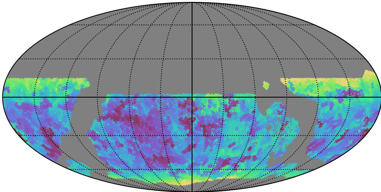
too_100_1v3.4_10yrs WFD all bands: Min seeingEff
