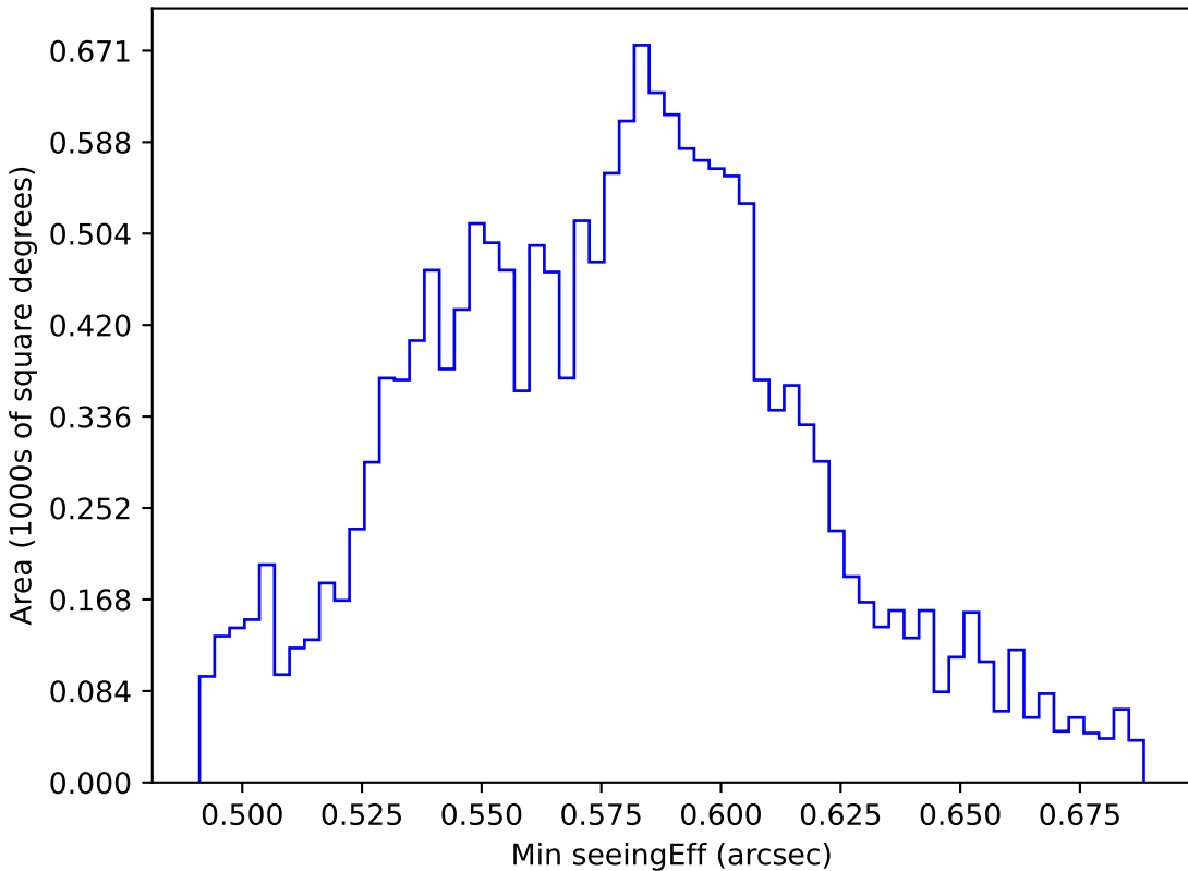
too_100_1v3.4_10yrs WFD all bands: Min seeingEff
