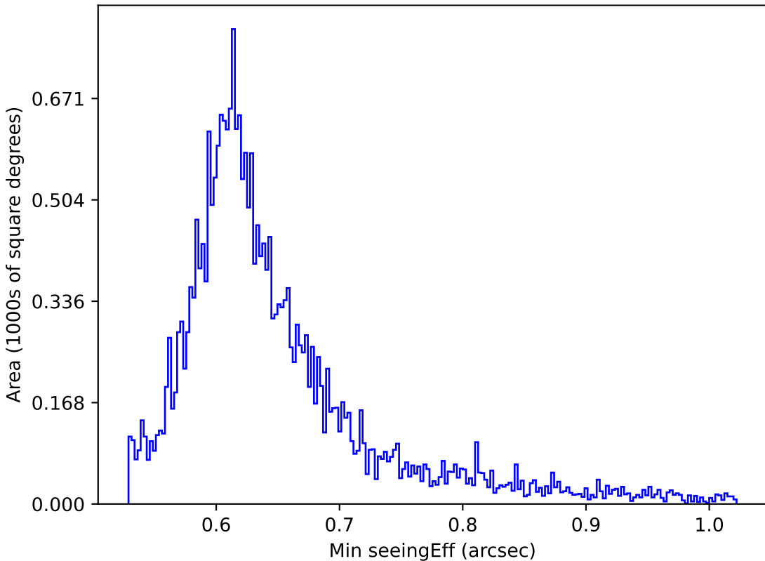
too_100_1v3.4_10yrs All sky z band: Min seeingEff
