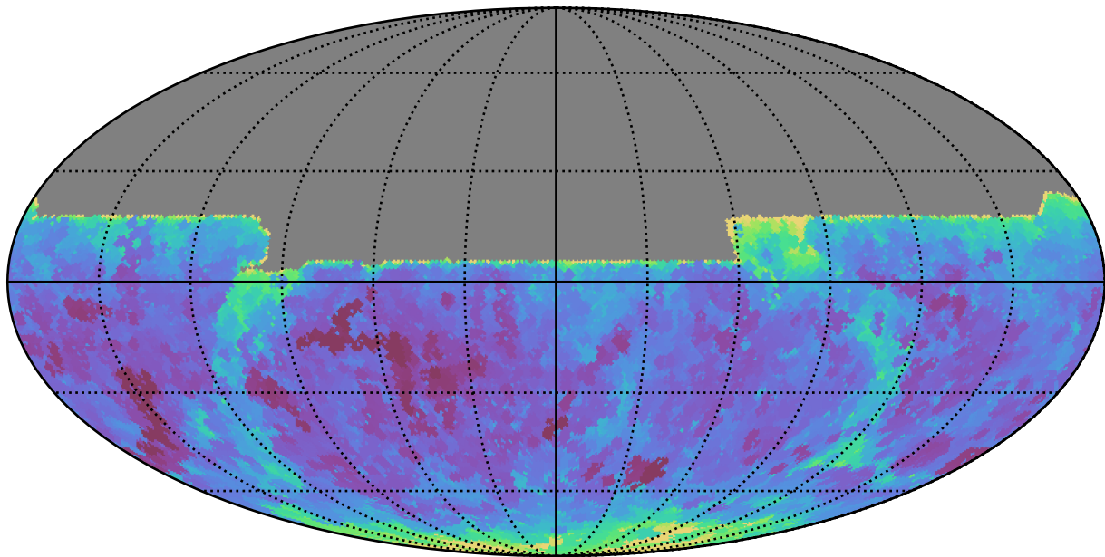
too_100_1v3.4_10yrs All sky y band: Min seeingEff
