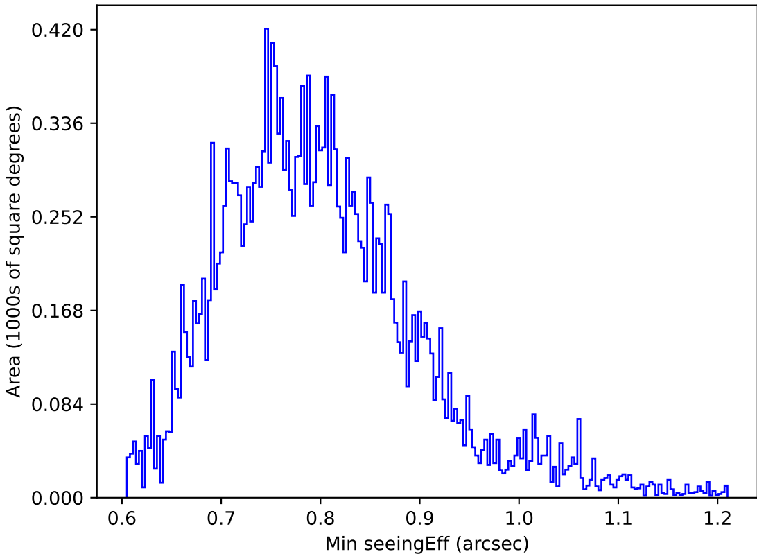
too_100_1v3.4_10yrs All sky u band: Min seeingEff
