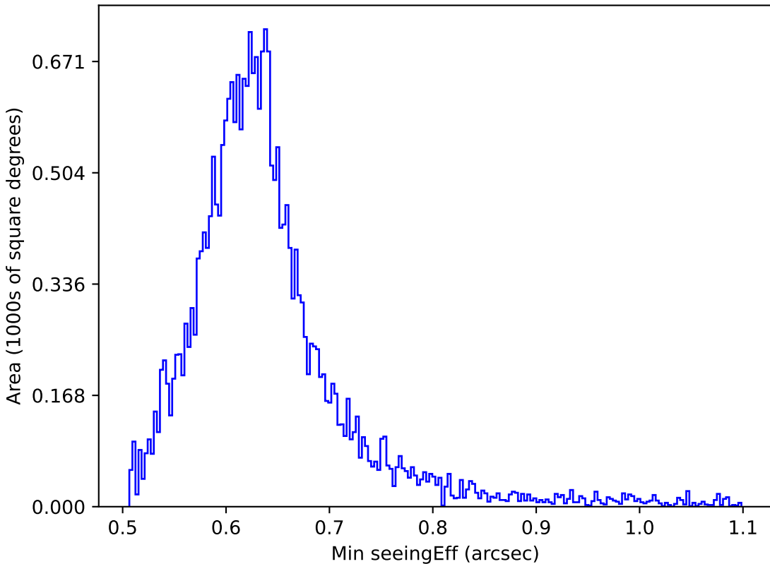
too_100_1v3.4_10yrs All sky r band: Min seeingEff
