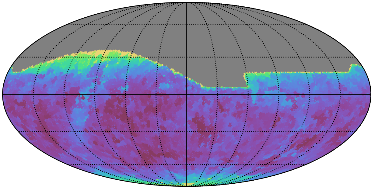
too_100_1v3.4_10yrs All sky i band: Min seeingEff
