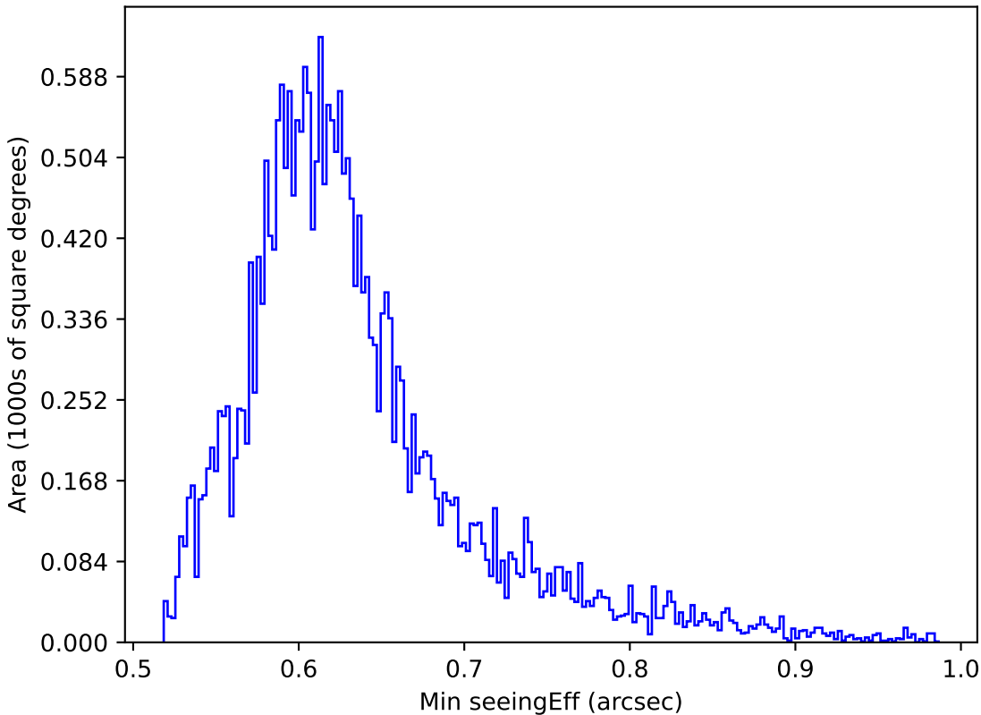
too_100_1v3.4_10yrs All sky i band: Min seeingEff
