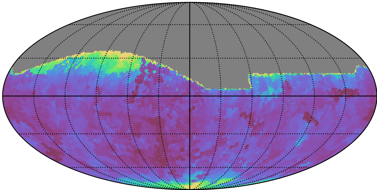
too_100_1v3.4_10yrs All sky g band: Min seeingEff
