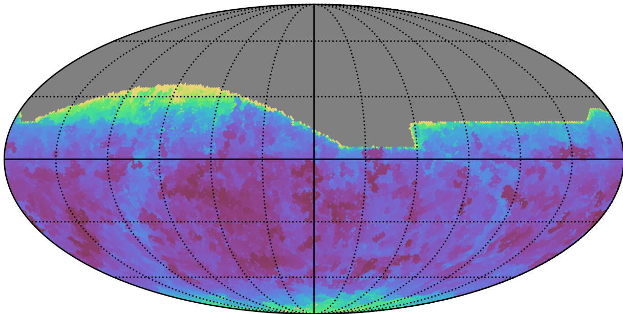
too_100_1v3.4_10yrs All sky all bands: Min seeingEff
