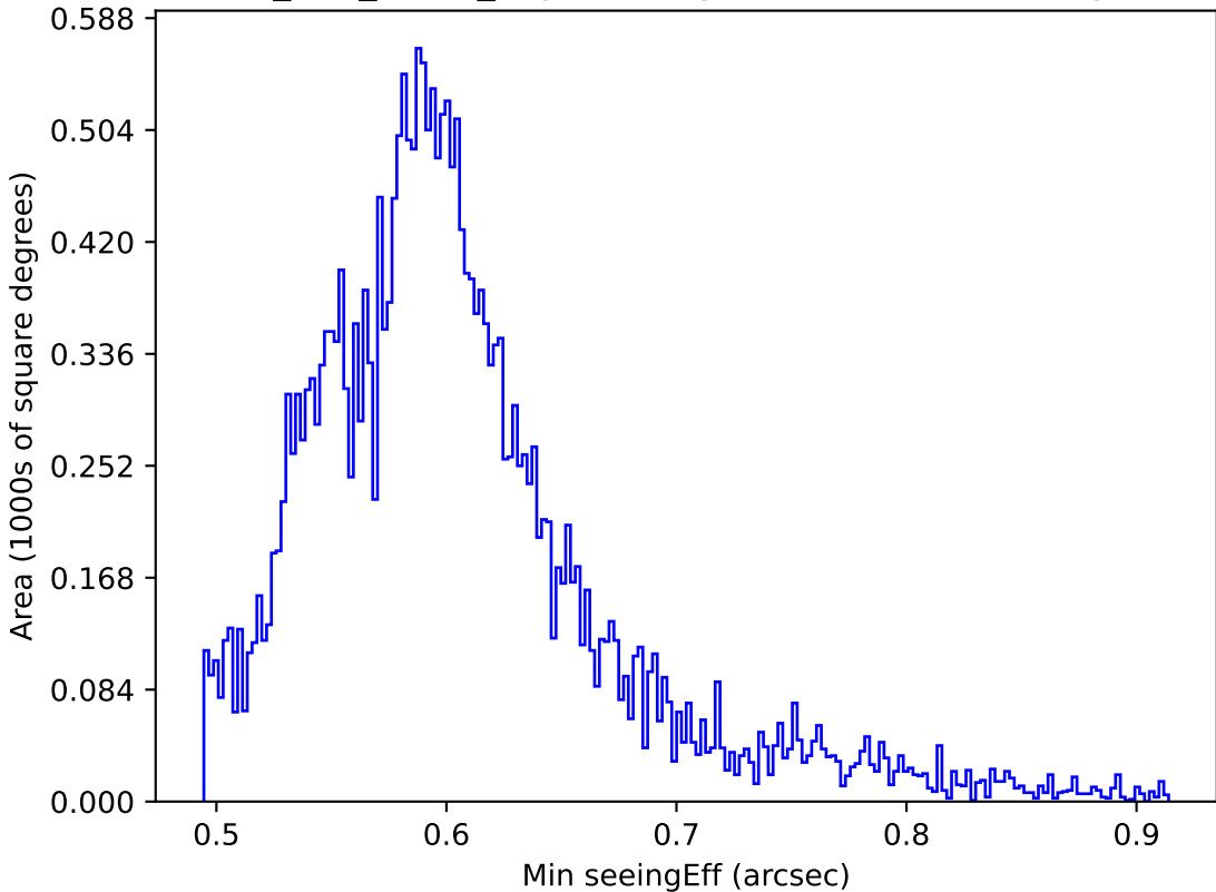
too_100_1v3.4_10yrs All sky all bands: Min seeingEff
