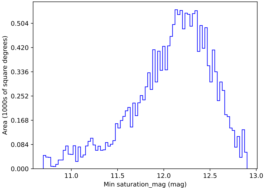
too_100_1v3.4_10yrs WFD z band: Min saturation_mag
