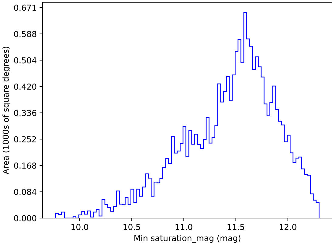
too_100_1v3.4_10yrs WFD u band: Min saturation_mag
