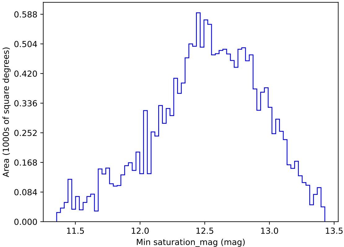
too_100_1v3.4_10yrs WFD r band: Min saturation_mag
