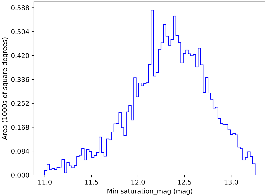
too_100_1v3.4_10yrs WFD i band: Min saturation_mag
