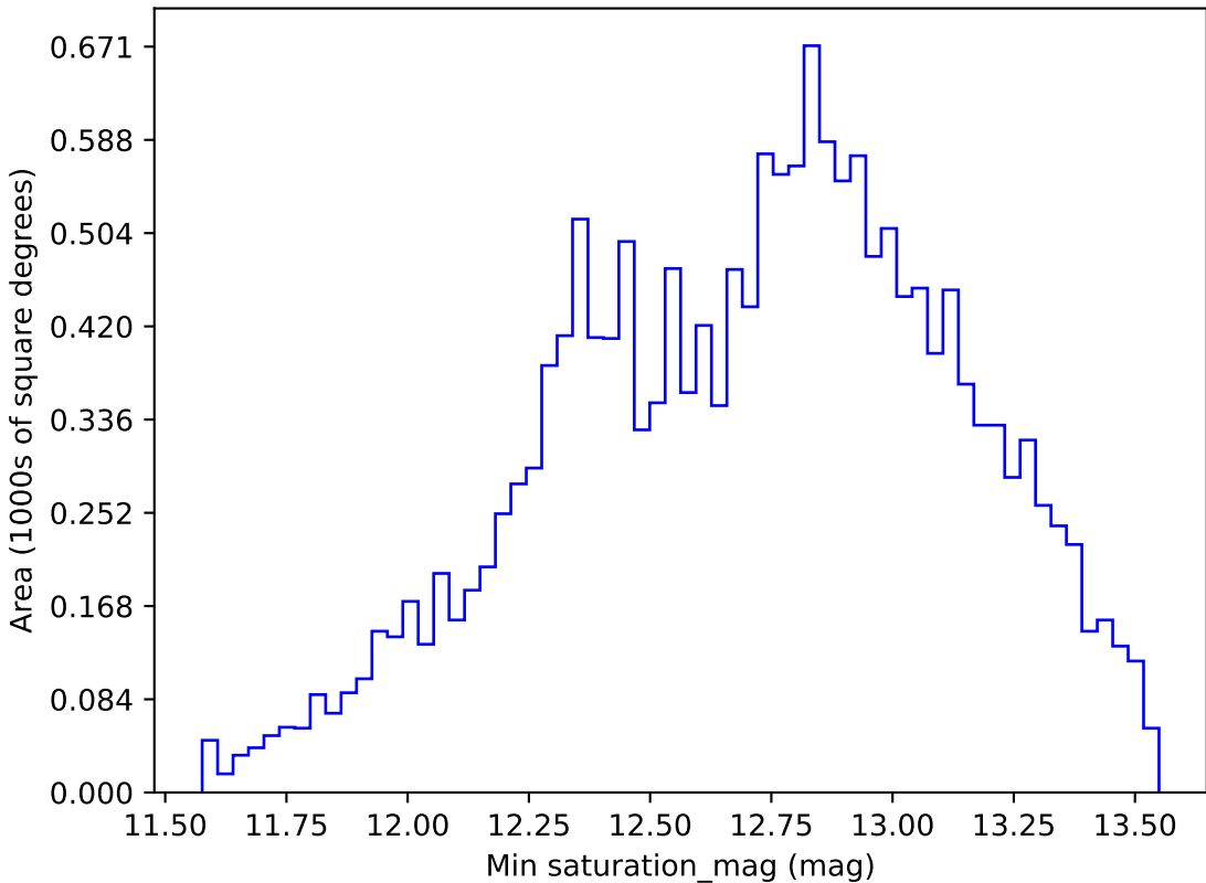
too_100_1v3.4_10yrs WFD g band: Min saturation_mag
