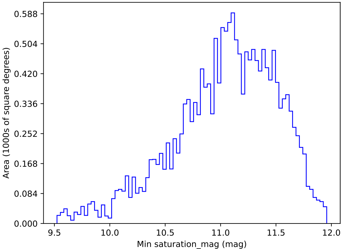
too_100_1v3.4_10yrs WFD all bands: Min saturation_mag
