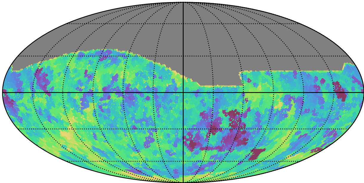
too_100_1v3.4_10yrs All sky z band: Min saturation_mag
