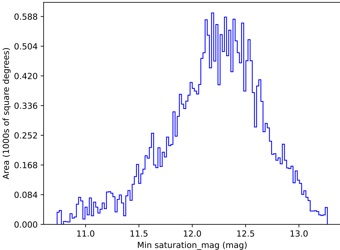
too_100_1v3.4_10yrs All sky z band: Min saturation_mag
